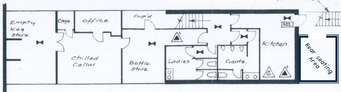
LOWER GROUND FLOOR PLAN.
